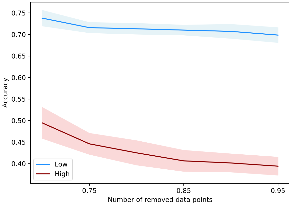
DataAttrOpt(10000, 0.1, 15, best, +b, alpha=best) - adult
